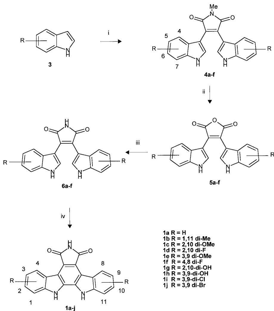
Scheme 1. Synthesis of indolocarbazoles. Reagents: (i) a. EtMgBr, THF, benzene b. 2 , THF, benzene; (ii) KOH, MeOH or dioxan; (iii) NH 4 OAc, 140 °C; (iv) DDQ, PTSA, toluene, 100 °C for examples 1a–1e , hv, iodine, isopropanol for example 1f . For conversions 1c into 1g and 1e into 1h , pyridine hydrochloride, 120 °C. For conversion 1a into 1i , N -chlorosuccinimide, MeCN. For conversion 1a into 1j , N -bromosuccinimide, MeCN.
