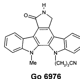
Figure 3. Structure of Go 6976.
