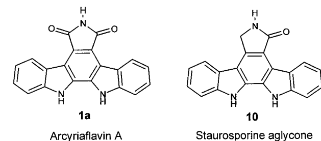
Figure 1. Structures of Arcyriaflavin A and Staurisporine aglycone.
